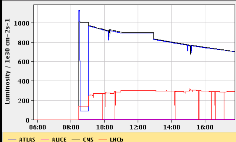
Instantaneous Luminosity
