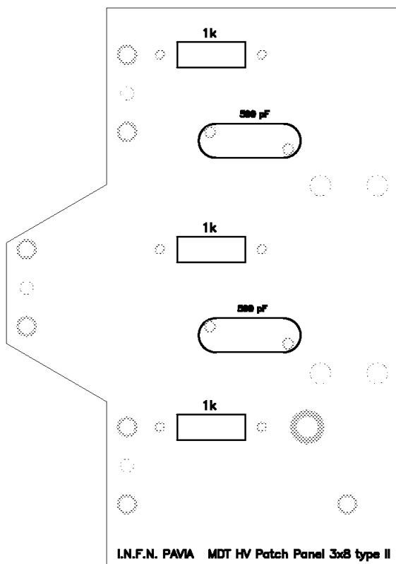
Patch panel for hedgehog type II
