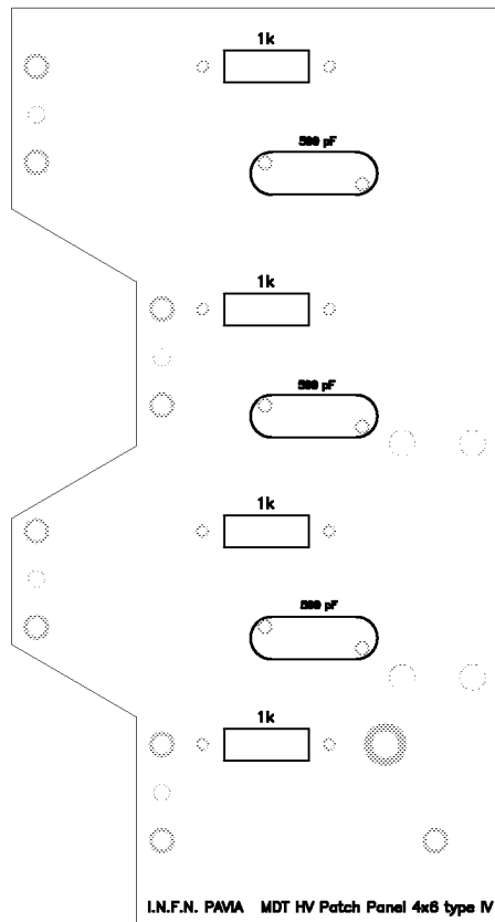
Patch panel for hedgehog type IV
