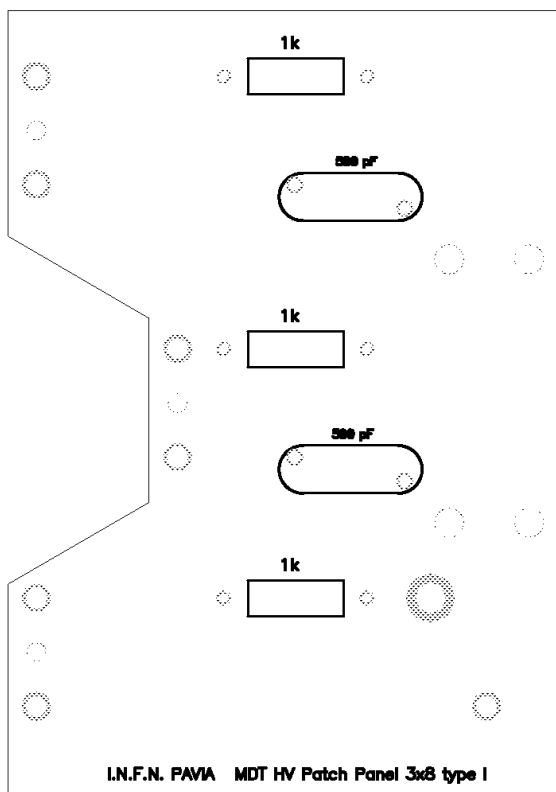
Patch panel for hedgehog type I
